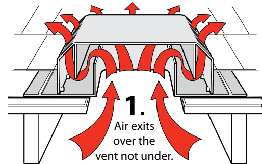
Interior baffle shield
